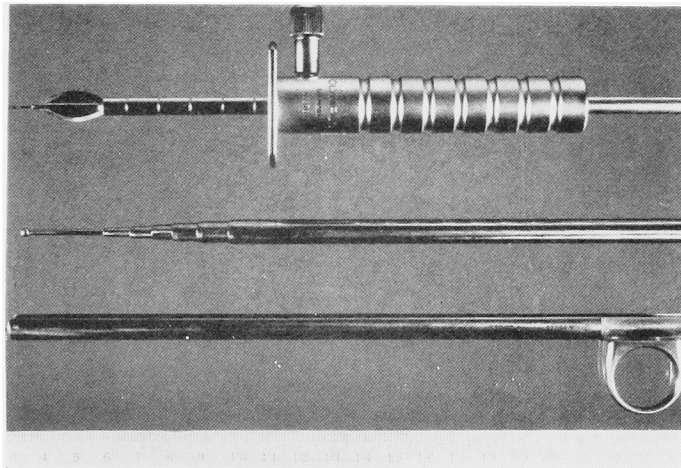
Fig. 3. Tools for dilation of nephrostomy tract, fascia cutter (upper), telescoping dilation set (middle) and slotted cannula (lower).
