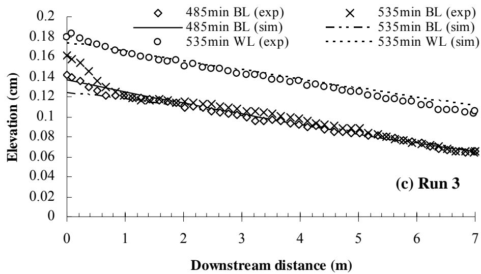
Fig. 4.66 Experimental and simulation results on bed surface and water surface
