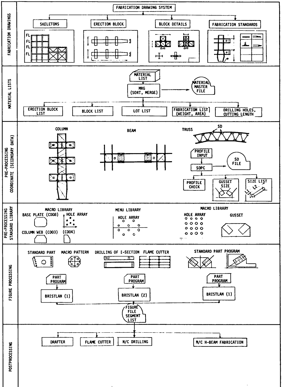
Fig. 3-26 N/C System in Building Frame
