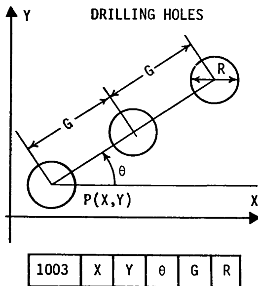
Fig. 3-7 Segment Lists (Expression of Figures)
