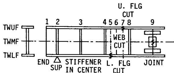
Fig. 3-6 Secondary Data Structure
