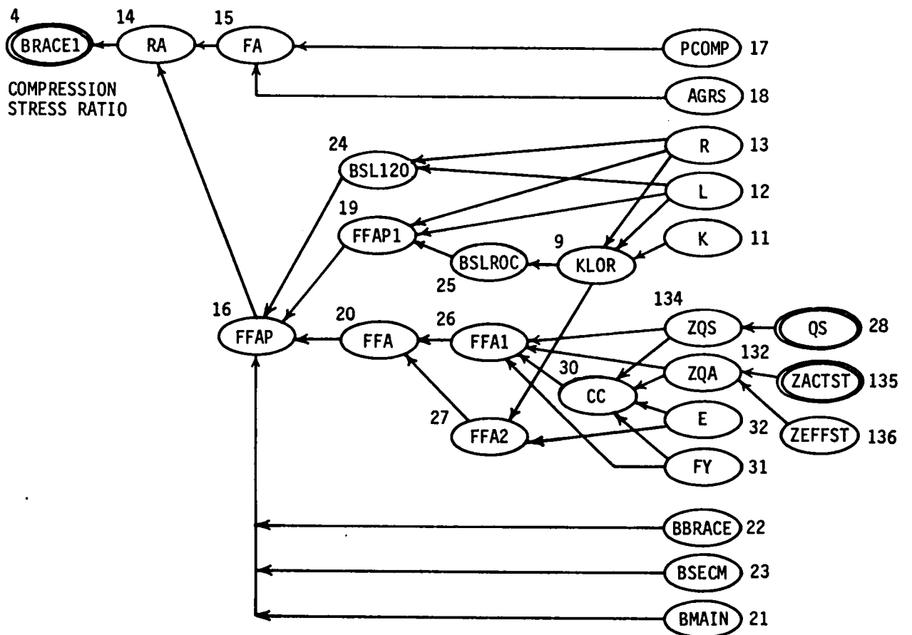
Fig. 2-6 Networks of BSL200 and BRACE1 (the AISC)
