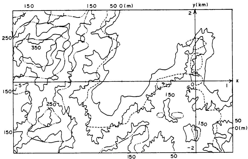
Fig. 2.19 Comparison of simulated terrain and real terrain when \theta = -90 deg. Contour line of real terrain ; —, contour line of simulated terrain ; .....= elevation of 50 m, - - - - = elevation of 150 m, - · - · = elevation of 250 m, - · · - = elevation of 350 m.
