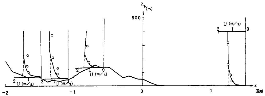
Fig. 2.37 Calculated and measured mean horizontal wind profiles over a real terrain form model. - - - - IPFM, — IQPFM, ● field experiment.
