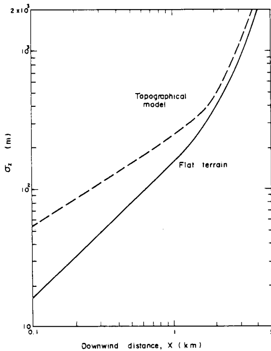
Fig. 3.17 Growth of vertical plume width.
