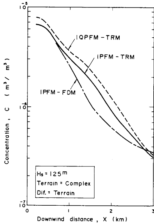
Fig. 3.27 Comparison of Gaussian plume trajectory model with FDM model (1).
