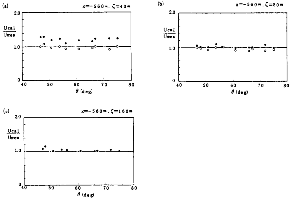
Fig. 2.38 Comparison of numerical calculations of wind velocities with field experiment data in presence of a real terrain form model (1).
