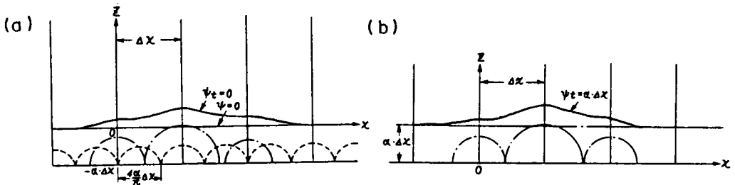
Fig. 2.5 Streamline simulating terrain boundary. The chained and dotted semicircles denote two-dimensional doublets.
