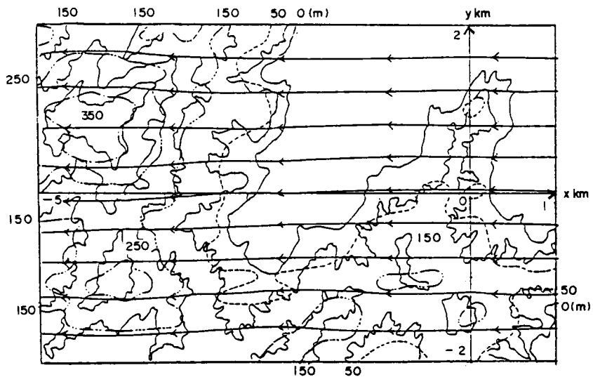
Fig. 2.16 Calculated streamlines.
