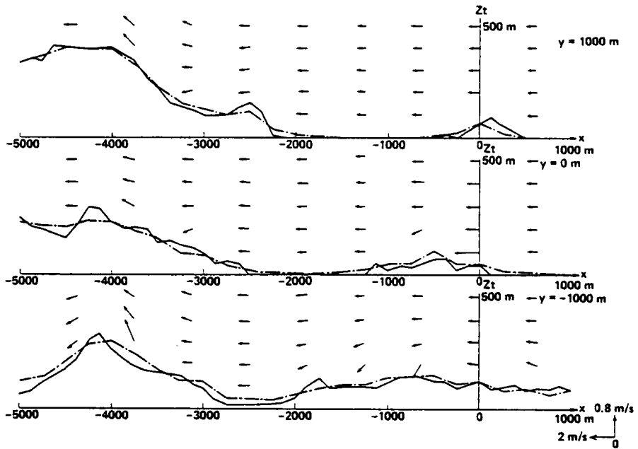
Fig. 2.14 Comparison of simulated terrain and real terrain and vertical vectors of calculated winds. The real terrain is denoted by solid lines while the simulated terrain is denoted by chained lines. Arrows denote the vertical vectors of calculated winds. The wind direction is \theta = 90 \text{ deg} .
