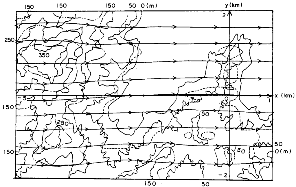
Fig. 2.21 Calculated streamlines.
