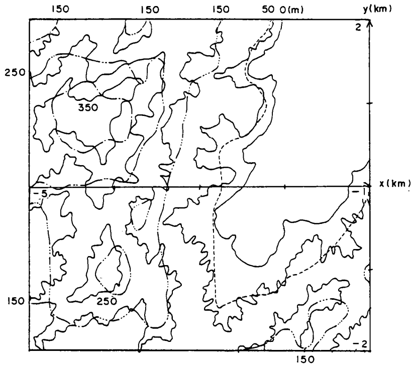
Fig. 2.18 Comparison of simulated terrain and real terrain when \theta = 0 deg. Contour line of real terrain ; —, contour line of simulated terrain ; .....= elevation of 50 m. — · — · = elevation of 150 m, — · — · = elevation of 250 m, — · — · = elevation of 350 m.
