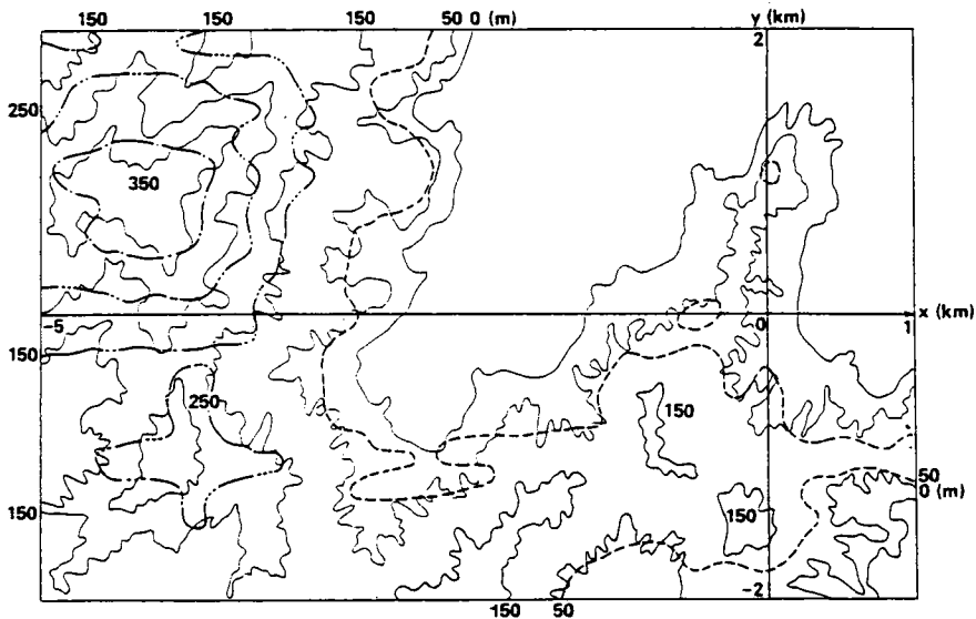
Fig. 2.11 Comparison of simulated terrain and real terrain. The correction factor c_{ij} is set to 1.0 at each grid point. Contour line of real terrain ; —, contour line of simulated terrain ; ..... = elevation of 50 m, — · — · — = elevation of 150 m, — · — · — = elevation of 250 m, — · — · — = elevation of 350 m.
