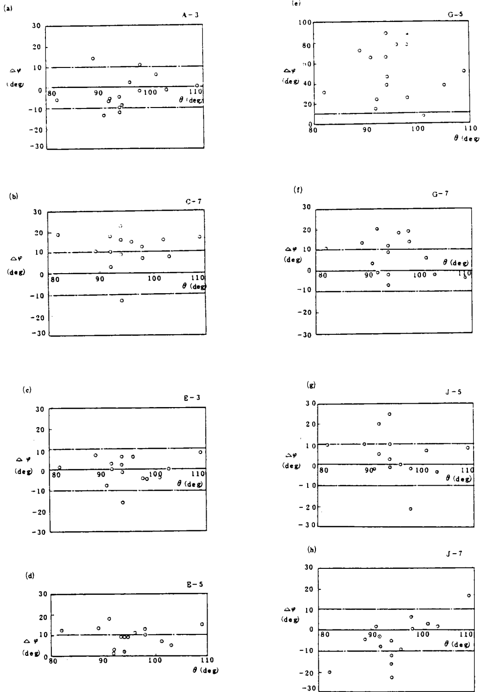
Fig. 2.31 Difference between calculated wind direction by IPFM and measured one.
