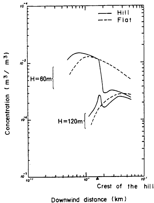
Fig. 3.7 Calculated downwind concentration distributions over a steep hill.
