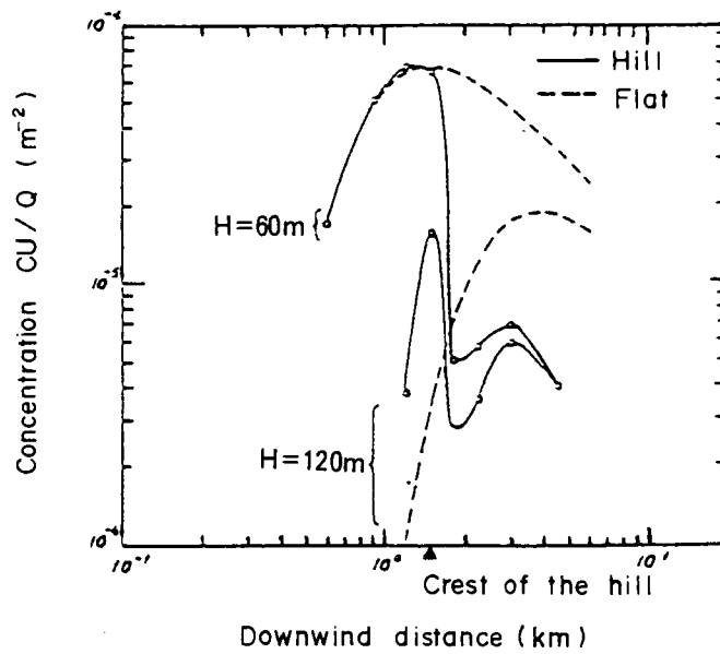
Fig. 3.9 Wind tunnel experimental results of downwind concentration distributions over a step hill.
