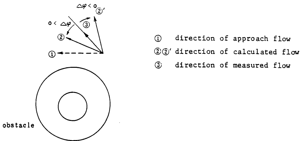
Fig. 2.32 Conceptual representation of the determination of \Delta\phi (difference between calculated wind direction and measured one).
