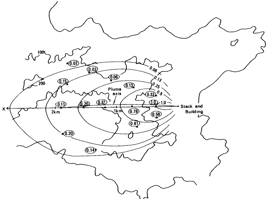
Fig. 3.22 Comparison of calculation result of surface concentrations with field experimental data in presence of the real terrain form model (Case 3).
