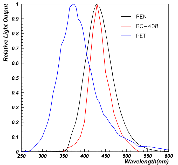
Fig. 3: Emission spectra of polyethylene naphthalate (PEN; black line), commercial organic scintillator (BC-408; red line) and a plastic bottle (PET; blue line).
