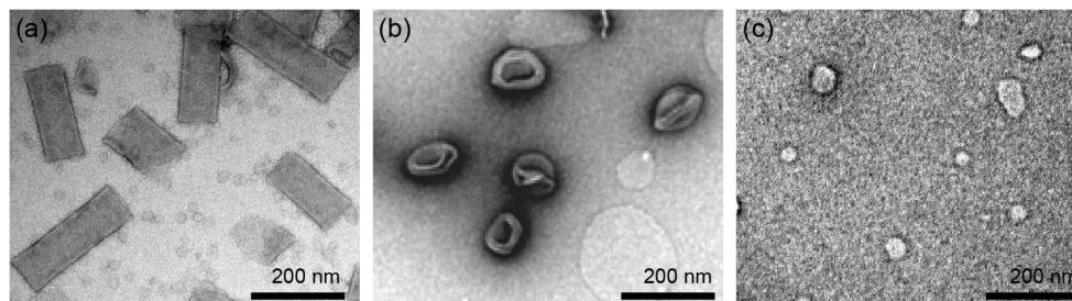
Figure 5. TEM images (negative staining with uranyl acetate; (a–c)) of molecular assemblies from single component of helical polypeptides S24L14 ; (a), S22L16 ; (b) and S25L20 ; (c). The molecular assemblies were prepared in a 10 mM Tris-HCl buffer (pH 7.4) (1 \mu\text{mol/mL} ) by the ethanol injection method after heat treatment at 90 °C for 1 h. The scale bars are 200 nm.
