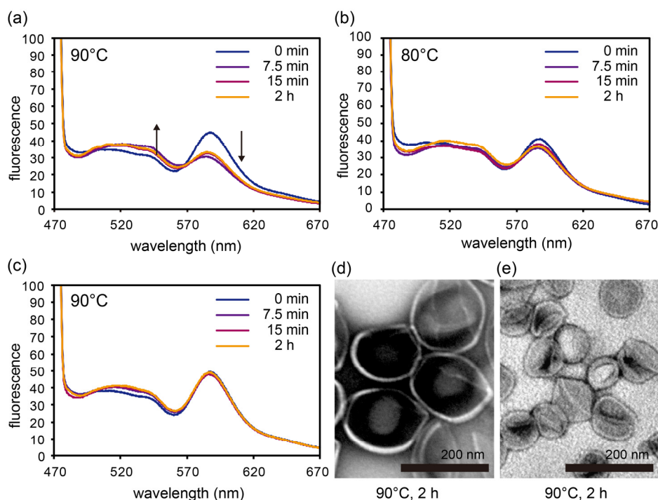
Figure 2. Emission spectra from a mixture of DL vesicles and DL vesicles containing of 0.25 % NBD-PE and 0.25 % Rho-PE upon heating (a); at 90 °C and (b); at 80 °C, and (c); from a mixture of L16 vesicles and L16 vesicles containing 0.25 % NBD-PE and 0.25 % Rho-PE upon heating at 90 °C. TEM images (negative staining with uranyl acetate) of (d); DL vesicles and (e); L16 vesicles after heating at 90 °C. The assembly suspensions were prepared in 10 mM Tris-HCl buffer (pH 7.4) (1 mg/mL) by the ethanol injection method.
