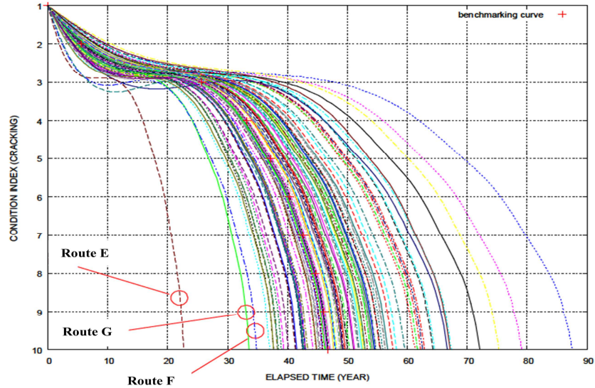
Figure 5.9 Deterioration Curve of Cracking along Route
