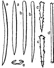
Text-fig. 6. Spicules of Clathria shirahama , n. sp.
