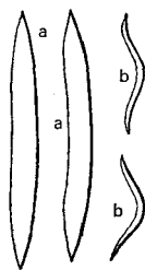
Text-fig. 3. Spicules of Callyspongia robusta (Ridley). a. oxeas \times 290 ; b. toxas \times 290 .
