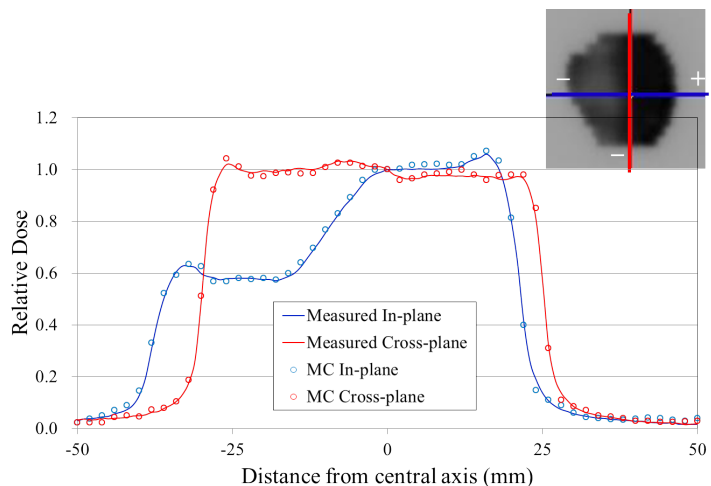
FIG. 11. Measured and simulated profiles of a step-and-shoot IMRT case. Dose was computed with a voxel resolution of 0.2 \times 0.2 \times 0.2 \text{ cm}^3 . Blue line = in-plane direction; red line = cross-plane direction.
