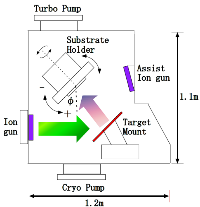
Fig. 1 Schematic view of ion beam sputtering system at KURRI.
