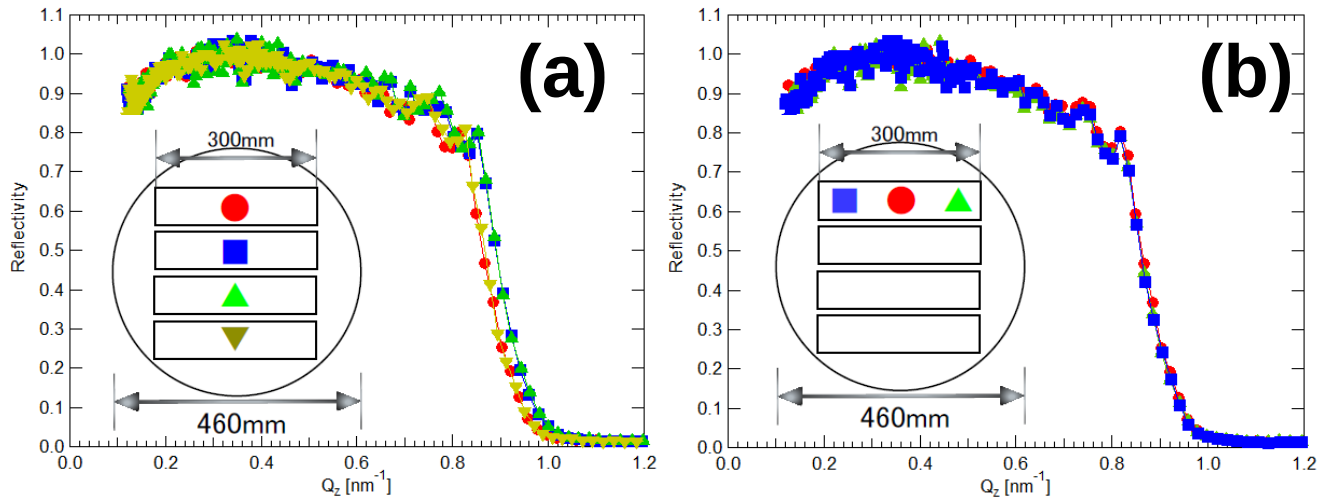
Fig. 6 Reflectivities of m=4 NiC/Ti supermirror with (a) the center of four mirrors, and (b) the left, center, and right of top mirror.
