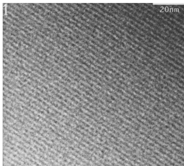
Fig. 2 Reflectivity of d=2.89 nm NiC/Ti multilayer mirror with 10000 layers; the cross-sectional TEM image. The inserted graph shows reflectivity of the second order. The incident neutron wavelength was 0.88 nm.
