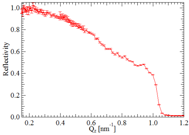
Fig. 8 Reflectivities of the m=5 NiC/Ti self-standing supermirror sheet affixed on glass plate.
