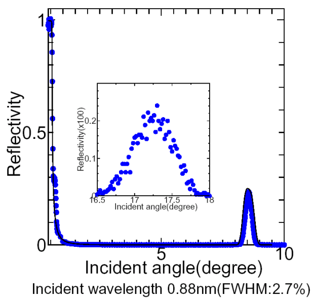
Fig. 2 Reflectivity of d=2.89 nm NiC/Ti multilayer mirror with 10000 layers; the cross-sectional TEM image. The inserted graph shows reflectivity of the second order. The incident neutron wavelength was 0.88 nm.
