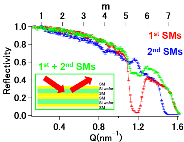
Fig. 4 Reflectivity of m=7 NiC/Ti supermirror stacking two mirrors, as shown in the insert.
