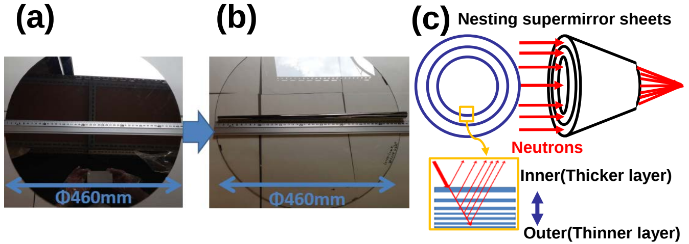
Fig. 7 Photograph of (a) m=5 NiC/Ti supermirror deposited on glass substrate and (b) the m=5 NiC/Ti self-standing supermirror peeling off from the glass substrate. (c) Schematic view of strong focusing device based on the nested axisymmetric supermirror sheets.
