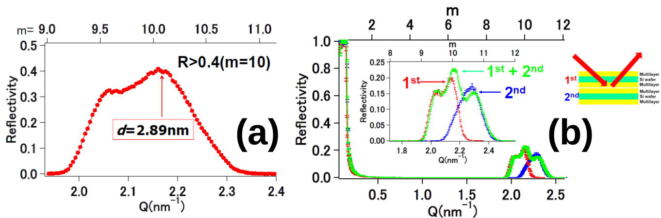
Fig. 3 Reflectivity of NiC/Ti stacking mirrors in with the following number of layers: (a) 85060; and (b) 10929(1 st ), 10336 (2 nd ), and 21265 (1 st +2 nd ), respectively.
