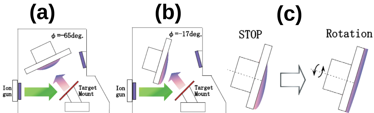
Fig. 5 Schematic illustration of thickness dependence on the tilt angle for (a) small, and (b) large samples in the case of stopping the substrate holder; (c) a schematic image of thickness dependence by rotating the substrate holder
