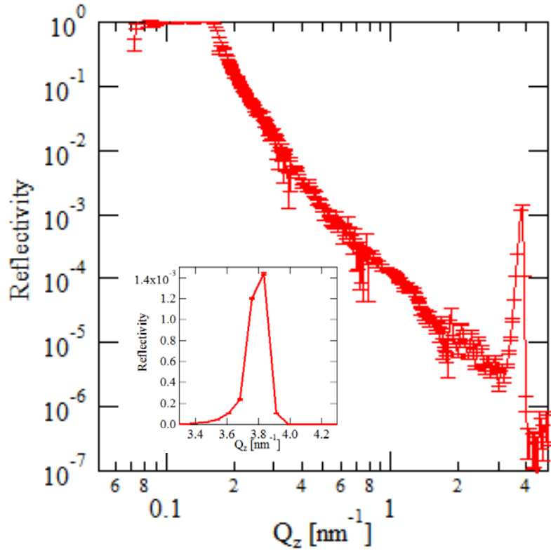
Fig.9 Reflectivity of d=1.65\text{nm} NiC/Ti self-standing multilayer mirror in which layers numbered 10000. The insert shows an enlarged view at 3.3 < Q_z < 4.3(\text{nm}) .
