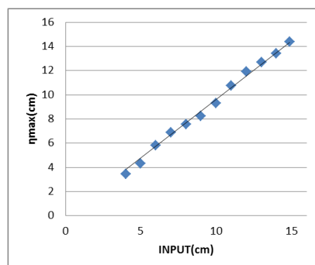
Fig.2 Relation between the maximum wave height and current velocity and INPUT value
