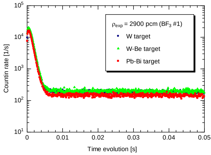
Fig. 3-5 Experimental results of time evolution on prompt and delayed neutron behaviors at position (10, U) of \text{BF}_3 detector #1 in Case I-3
