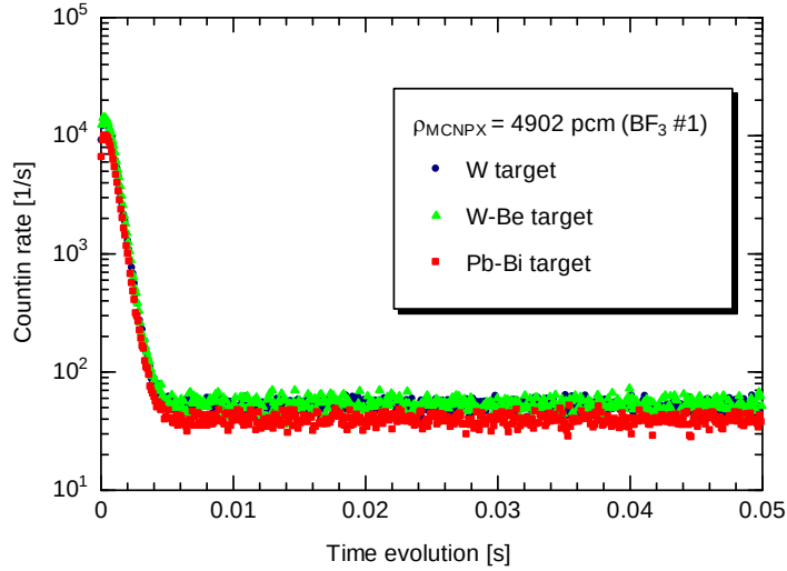
Fig. 3-6 Experimental results of time evolution on prompt and delayed neutron behaviors at position (10, U) of \text{BF}_3 detector #1 in Case I-5
