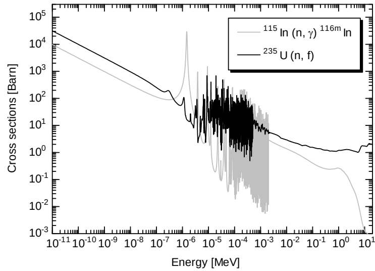
Fig. 3-3 Proportionality of cross sections of ^{115}\text{In} capture and ^{235}\text{U} fission reactions
