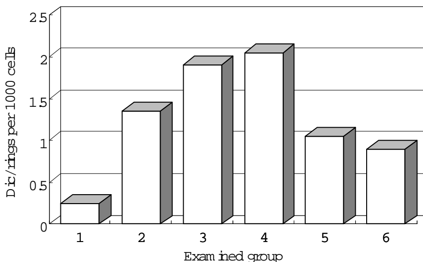
Fig. 2. The frequency of cells with dicentrics and centric ring chromosomes in the examined groups of the population of Muslyumovo (Chelyabinsk region). 1 - control group; 2 - all examined individuals; 3 - born before 1949; 4 - born in the period from 1949 to 1956; 5 - born in the period from 1957 to 1988; 6 - evacuated from other settlements.
