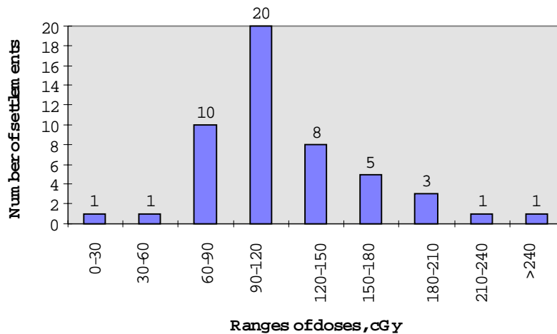
Fig. 3. Distribution of the number of settlements in the Lugny district according to thyroid irradiation doses for children born in 1986 (according to [3])
