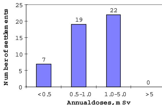
Fig. 1. Number of settlements of the Lugyny district which fit the criteria to be qualified for different zones of radioactive contamination (according to [2])
