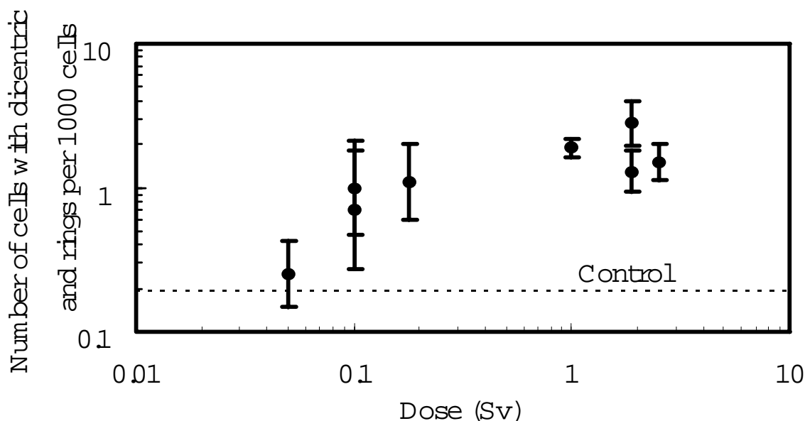
Fig. 1. The frequency of cells with dicentrics and centric ring chromosomes in the examined groups of the Altai population depending on the effective dose of irradiation caused by the nuclear explosion on the Semipalatinsk nuclear test site in 1949.
