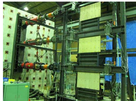
Figure 7. A steel wall with vertical slits is used as a hysteretic damper. Although the vertical slits change the mode of deformation from overall shear deformation to a series of flexural deformations and make the wall more energy dissipative, out-of-plane buckling yet occurs unless the wall is very thick. To delay such buckling even for thin walls, we enclose the wall by wood panel from both sides (top). The bottom picture shows a demonstration test of a three story planar frame in which such walls are installed. The walls are indeed energy dissipative.
