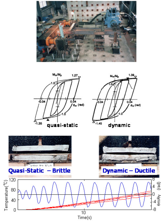
Figure 4. We looked into the effect of rate-of-loading on the performance by the application of dynamic loading to the connection (top). The two hysteresis loops (second top) show the results of quasi-static and dynamic loading. If anything, the dynamic loading exhibited more ductile behavior than the quasi-static loading. In fact, the fractured surfaces were more brittle in quasi-static loading (second bottom, left) than in dynamic loading (second bottom, right). A most plausible reason was the significant rise in temperature (bottom) during dynamic loading. These results were published as an article of ASCE Structural Journal. Fortunately, the article was awarded “ASCE Moisseif Award”.
