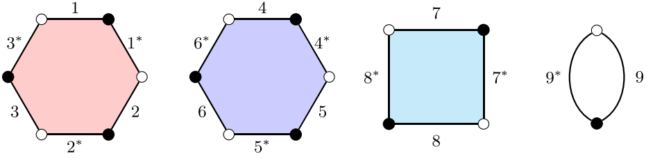
図2 (3, 3, 2, 1)-polygons
