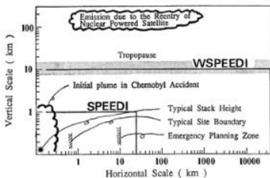
Figure 4 Spatial coverage of SPEEDI and WSPEEDI.
