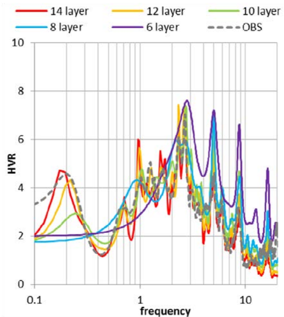
Fig. 19 Comparison of 1D theoretical earthquake HVSРs for the velocity model identified at MYG006 with different numbers of layers from the top as a parametric study. A broken line shows the observed HVSР. The original inverted structure has 14 layers down to the seismological bedrock (after Kawase et al., 2018).
