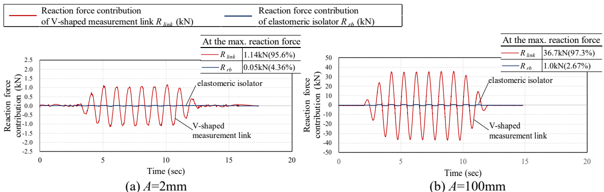
Fig. 15. Reaction force contribution with Elastic pin link.
