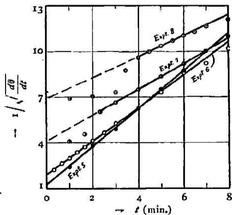
Fig. 6.—Expt. 8; \left[ \frac{1}{\sqrt{\frac{d\theta}{dt}}} - 6 \right] \sim t .
