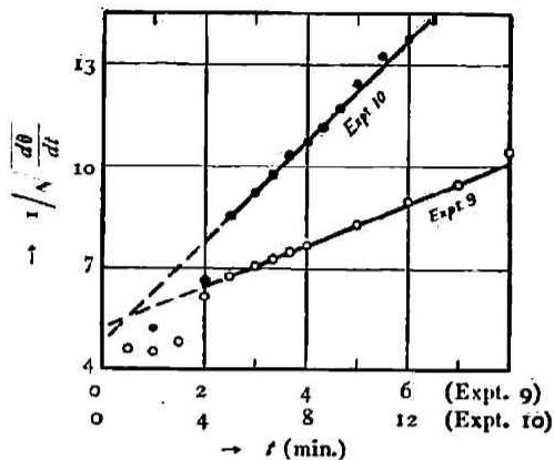
Fig. 9.—Salt effect.
