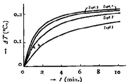
Fig. 2.—Influence of [II + ].
