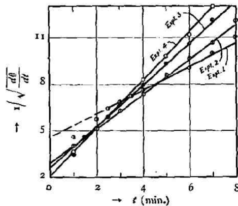
Fig. 4.—Influence of [H^+] .
