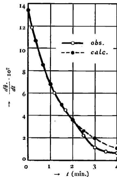
Fig. 12.—Expt. 12 (Pseudo-unimolecular).
