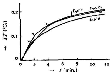
Fig. 8.—Salt effect.
