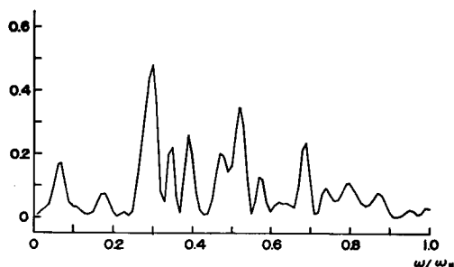
Fig. 5 Power spectral density of earthquake-type ground acceleration.
