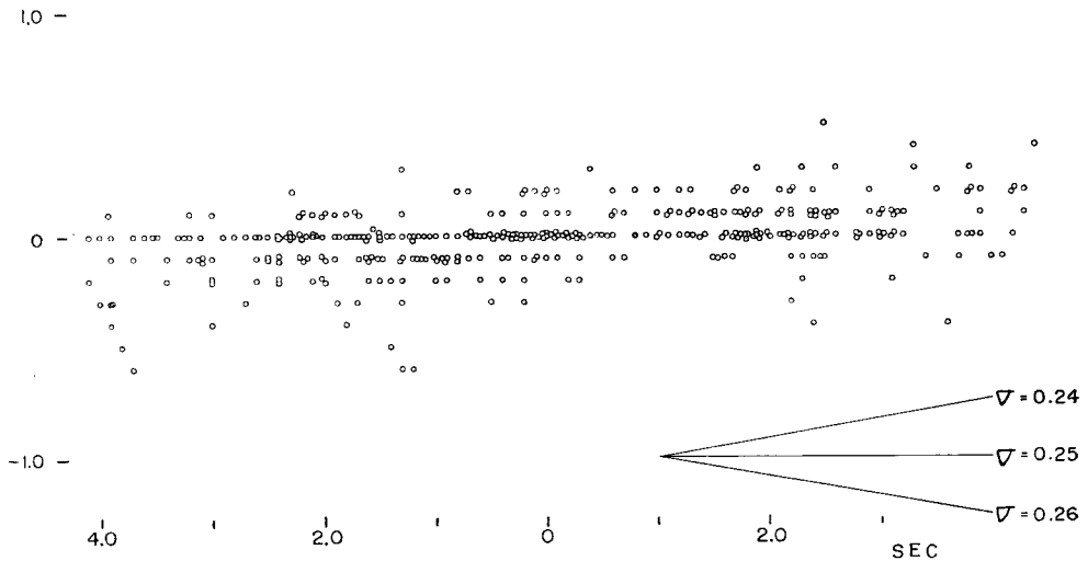
Fig. 1 Deviation of arrival time from best fitted line equivalent to Poisson's ratio \sigma = 0.25 on P arrival time versus S-P time graph. This figure is superposed suitably for all earthquakes used in this paper.
