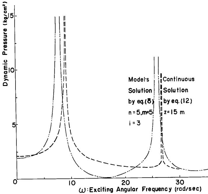
Fig. 9 Frequency Response of the Dynamic Pressure acting on Vertical Wall
