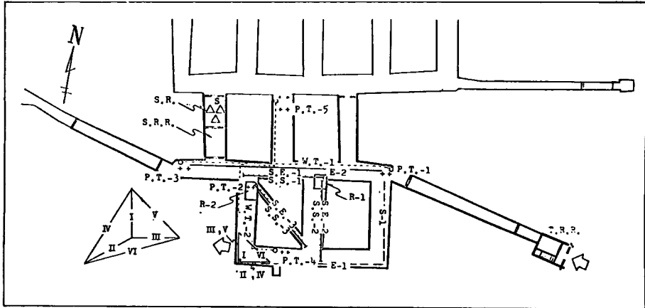
Fig. 1 Arrangement of instruments.
