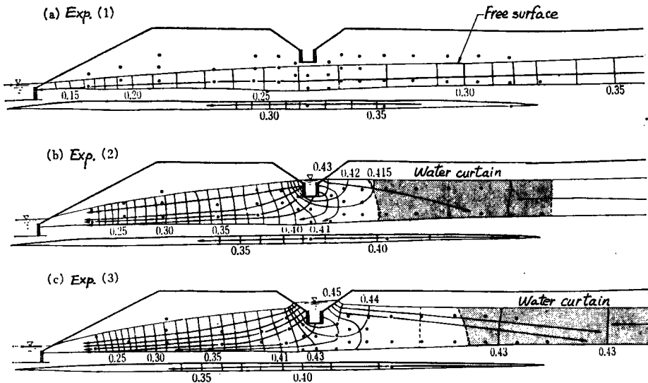
Fig. 11 Flow net in the steady state during the in-situ test.
