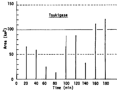
Fig. 16. The modified time-area-concentration diagram at Tsukigase.
