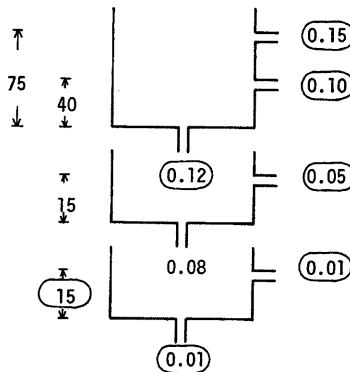
Fig. 9. The Tank model for Kohira basin.
