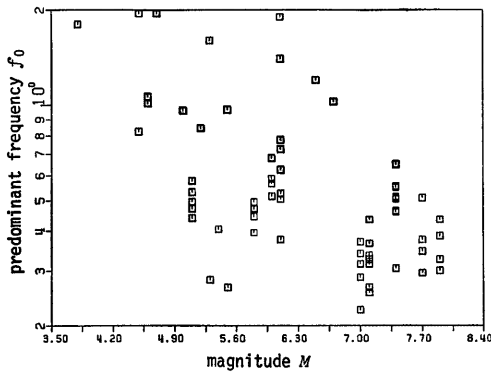
Fig. 11 Relation between predominant frequency f_0 of surface waves and earthquake magnitude M
