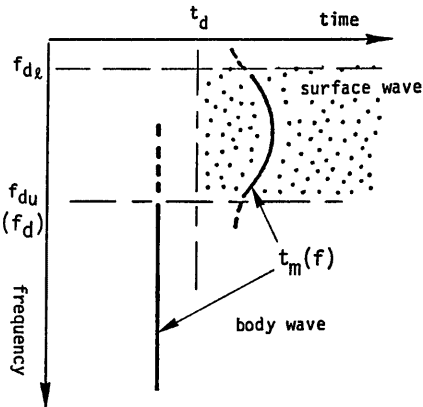
Fig. 1 Schematic description for peak time t_m(f) of evolutionary power spectra with separation parameters t_d , f_{d1} , and f_{d2} .
