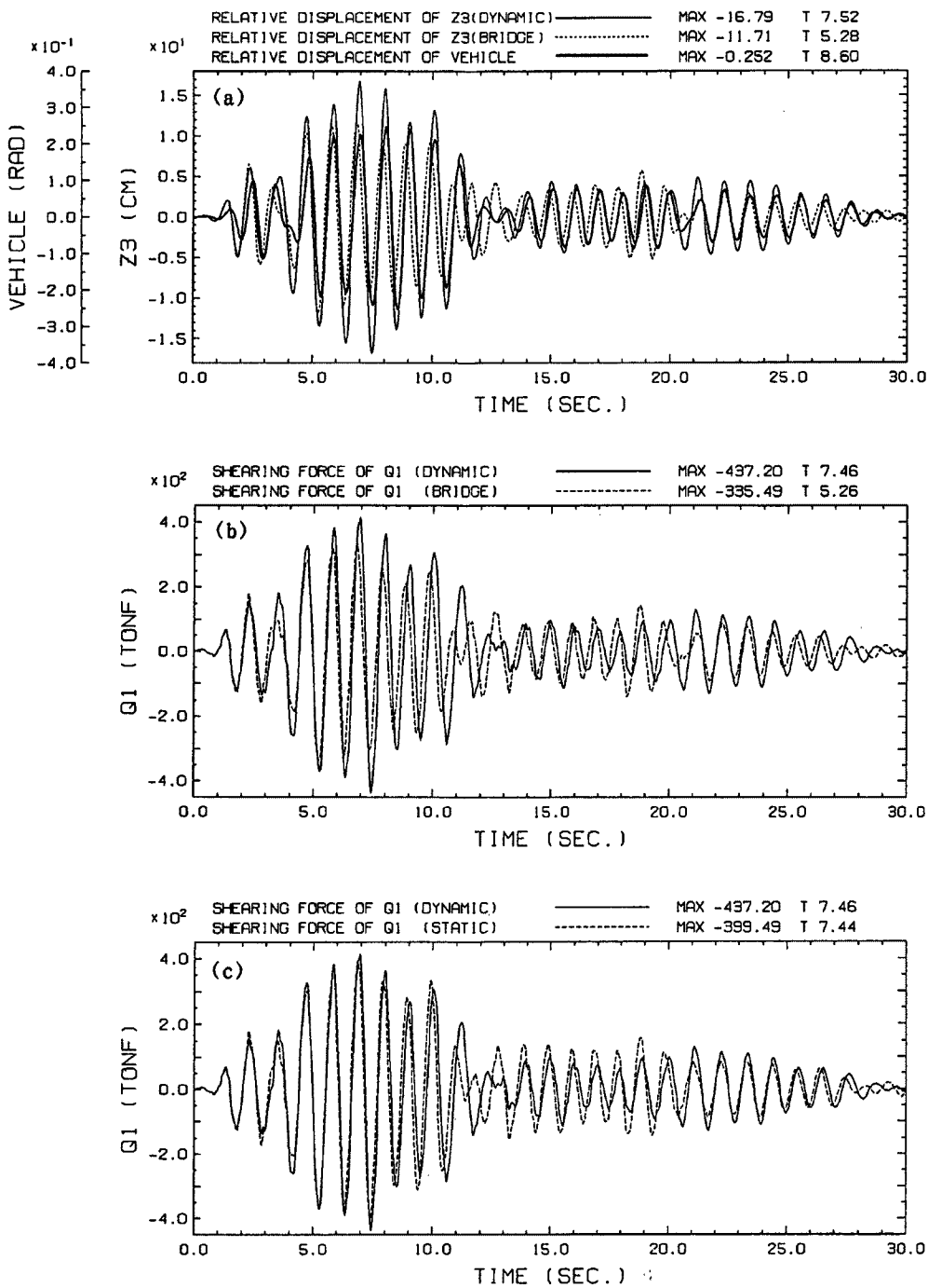
Fig. 15 (I). Time history of horizontal shear at foundation base (transverse; amplifying mode; input=CEQ4; phase delay=0.0; four vehicles; loading ratio r=0.75; sym. position).
