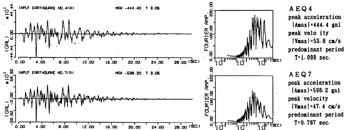
Fig. 8(a). Typical example of simulated ground motion group A.
