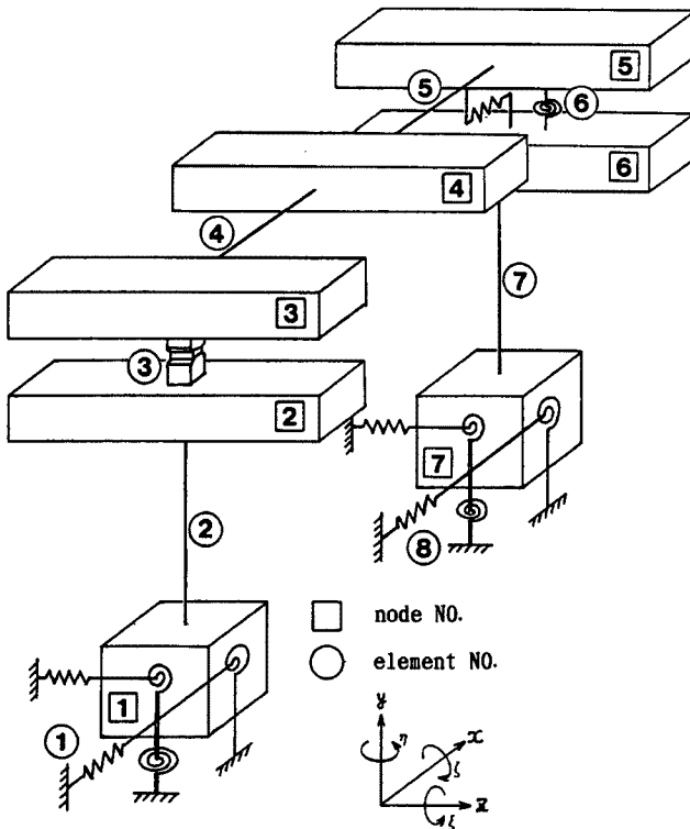
Fig. 2. Dynamic model of bridge.
