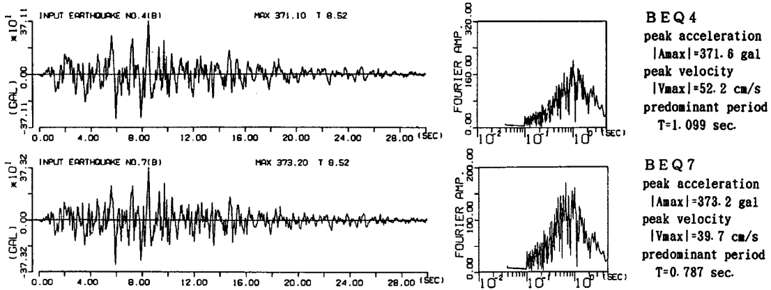
Fig. 8(b). Typical example of simulated ground motion group B.
