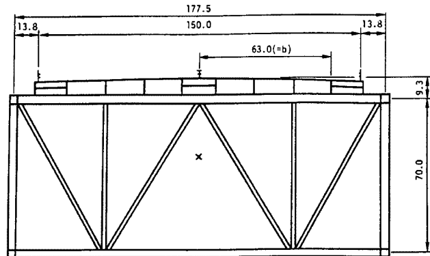
Fig. 5. Model of truss dfgirder section.
