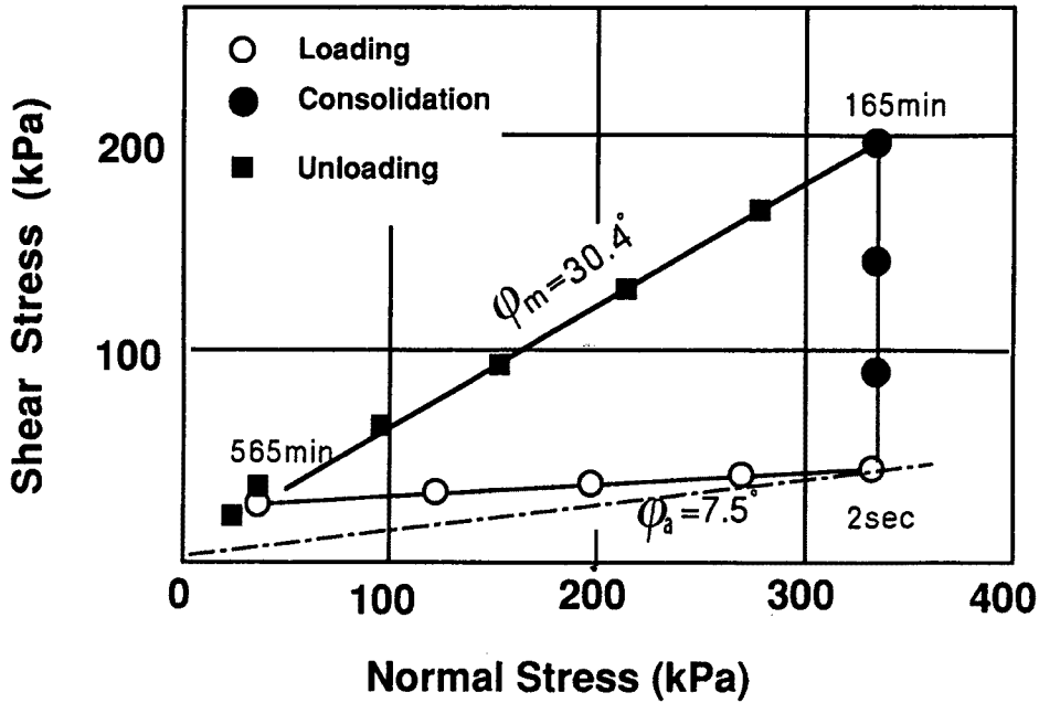
Fig. 7. Stress path of the rapid loading test (Sassa et al 17) . Sample: Saturated alluvium soil, e=0.49\sim 0.64 Shear speed: 6.2 cm/sec in rapid loading, 0.014 cm/sec in consolidation at 333 kPa, 0.014 cm/sec in unloading from 333 kPa.
