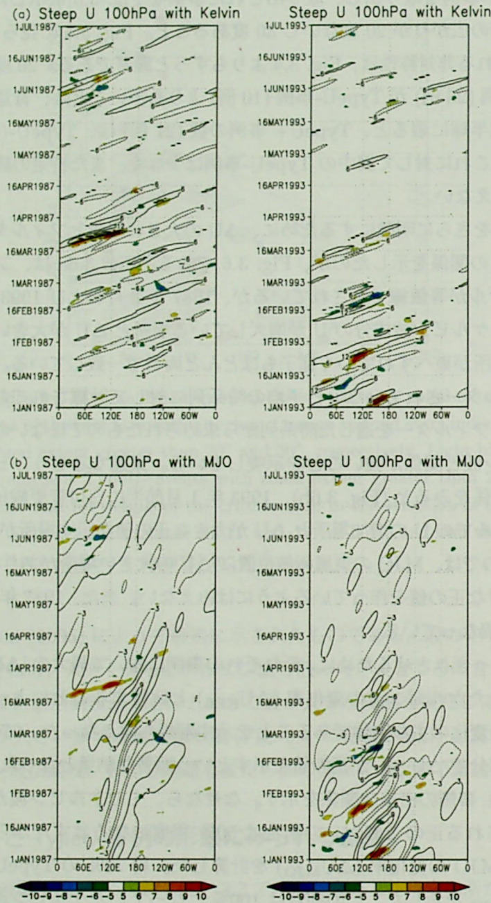
Fig. 3.6 Longitude-time sections of \Delta U at 0^\circ\text{N} during (a) January-June 1987 and January-June 1993 ( \text{m s}^{-1} \text{ day}^{-1} ). \Delta U is shown by colors. Filtered (a) Kelvin wave and (b) MJO are shown with contours. Contour levels are -18, -12, -6, 6, 12, 18 ( \text{m s}^{-1} ) in (a) and -9, -6, -3, 3, 6, 9 ( \text{m s}^{-1} ) in (b). Dashed line indicates the negative value.
