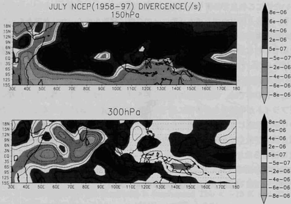
Fig. 1.8 Climatological (1958-97) Horizontal divergence ( s^{-1} ) at (upper) 150 hPa and (lower) 300 hPa in July in NCEP reanalysis. Contour interval is 2 \times 10^{-6} s^{-1} ; dashed lines show negative values.
