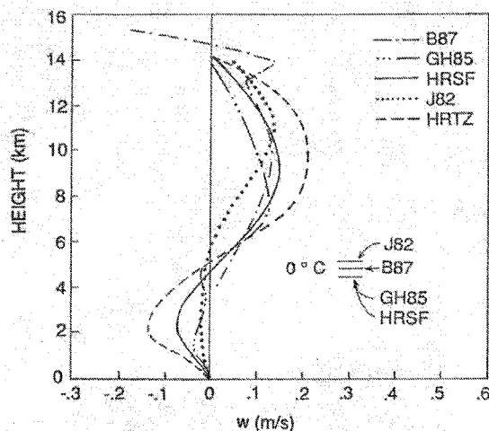
Fig. 4.2 Tropical oceanic and island stratiform-region vertical velocity profiles. The GH85 curve is from Gamache and Houze's (1985) composite sounding and aircraft wind analysis of the 12 September 1974 GATE squall line. The HR curves are from Houze and Rappaport's (1984) composite sounding and aircraft wind analysis of the 28 June 1974 GATE squall line; HRTZ is for the transition zone and HRSF is for the stratiform region proper. Curve J82 is from Johnson's (1982) rawinsonde analysis of Winter MONEX cloud clusters. The B87 curve is from the study of Balsley et al. (1988); it shows the two-year average vertical velocity during periods of light rain (0.5-12.7mm/h) at Pohnpei in the tropical western Pacific. (Figure and caption are taken from Houze 1989)
