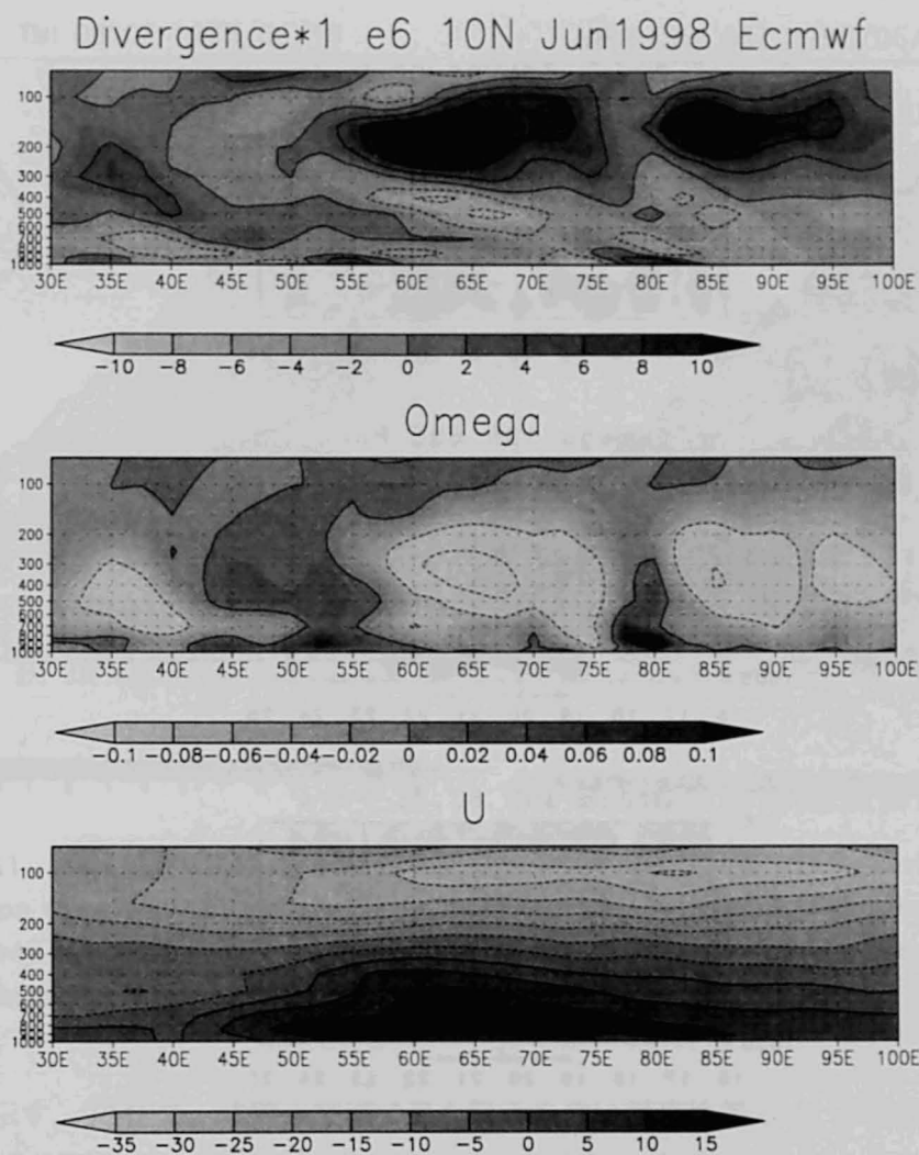
Fig. 1.9 Monthly mean of (upper) horizontal divergence ( 10^{-6} \text{ s}^{-1} , contour interval 4 \times 10^{-6} \text{ s}^{-1} ), (b) vertical p-velocity ( \text{Pa s}^{-1} , contour interval 0.1 \text{ Pa s}^{-1} ), and (c) zonal wind ( \text{m s}^{-1} , contour interval 5 \text{ m s}^{-1} ) at 10^\circ\text{N} in June 1998 in ECMWF reanalysis. Dashed lines show negative values.
