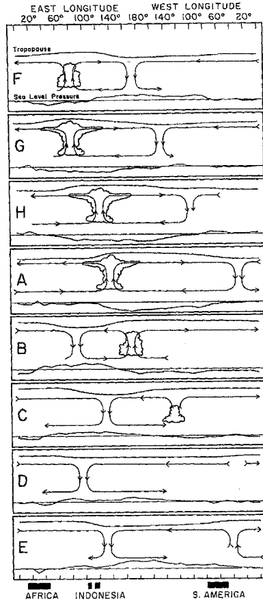
Fig. 1.2 Schematic depiction of the time and space (zonal plane) variations of the disturbances associated with the 40-50-day oscillation. Dates are indicated symbolically by the letters at the left of each chart and correspond to dates associated with the oscillation in Canton's station pressure. The letter A refers to the time of low pressure at Canton and E is the time of high pressure there. The other letters represent intermediate times. The mean pressure disturbance is plotted at the bottom of each chart with negative anomalies shaded. The circulation cells are based on the mean zonal wind disturbance. Regions of enhanced large-scale convection are indicated schematically by the cumulus and cumulonimbus clouds. The relative tropopause height is indicated at the top of each chart. (Figure and caption are taken from Madden and Julian 1972)
