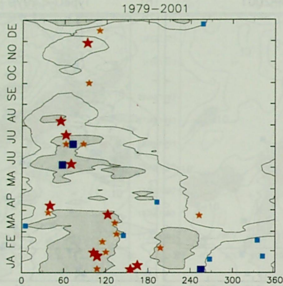
Fig. 3.5 Longitude( ^{\circ} E)-time distribution of cases with large zonal extent and eastward movement of the rapid transition region. Orange and red stars indicate TypeU+ events with zonal extent greater than 20^{\circ} and 30^{\circ} , respectively. Light blue and dark blue squares represent TypeU- events with zonal extent greater than 20^{\circ} and 30^{\circ} , respectively. See text for details of the criteria used in the selection of events. Solid lines indicate Kelvin wave variance of 11 and 14 \text{ m}^2 \text{ s}^{-2} , and the shaded region represents variance of greater than 14 \text{ m}^2 \text{ s}^{-2} .
