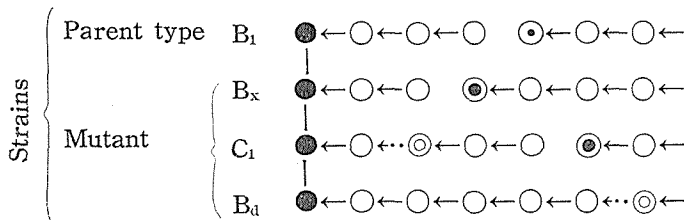
Fig. 2 Enzyme block in pyocyanine synthesis of mutant strain.
