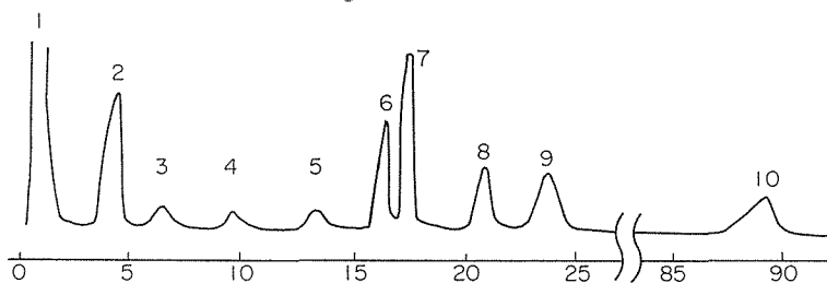
Fig. 1. A typical glc of the reaction mixture. (90°C, 4 hours in Table 1.)
