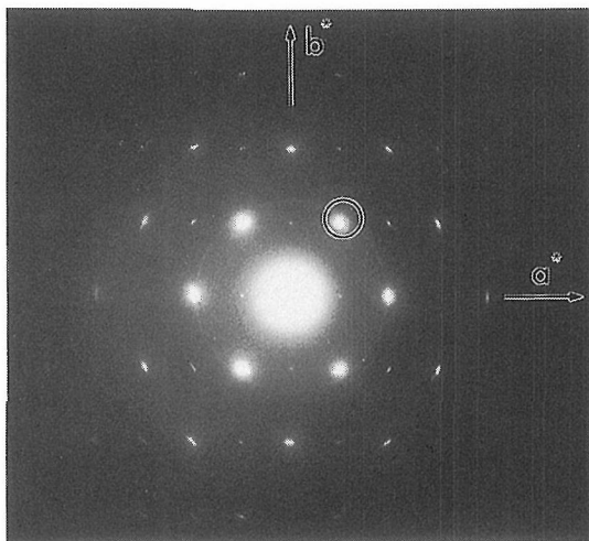
Fig. 4 Electron diffraction pattern of PE single crystal decorated with P3HT whiskers. The diffraction spots show the hk0 net pattern of PE. The diffraction ring predominantly stems from the 020 planes of P3HT. The circle in the figure shows the position of objective aperture for the dark-field image in Fig. 5.
