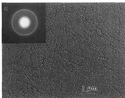
Fig. 1 TEM image of P3HT whiskers (b) and electron diffraction pattern (a). The whiskers were grown from a 0.05 wt % P3HT/cyclohexanone solution. Shaded with Pt in order to increase contrast.
