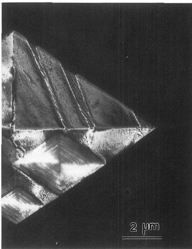
Fig. 5 Dark-field image of PE single crystal decorated with P3HT whiskers. The whiskers having a direction parallel to the vector from the origin of the diffraction pattern to the circle in Figure 4 appear in this photomicrograph. Thus, the P3HT whiskers grown onto the lateral surface of PE single crystal are normal to (110) planes of PE.
