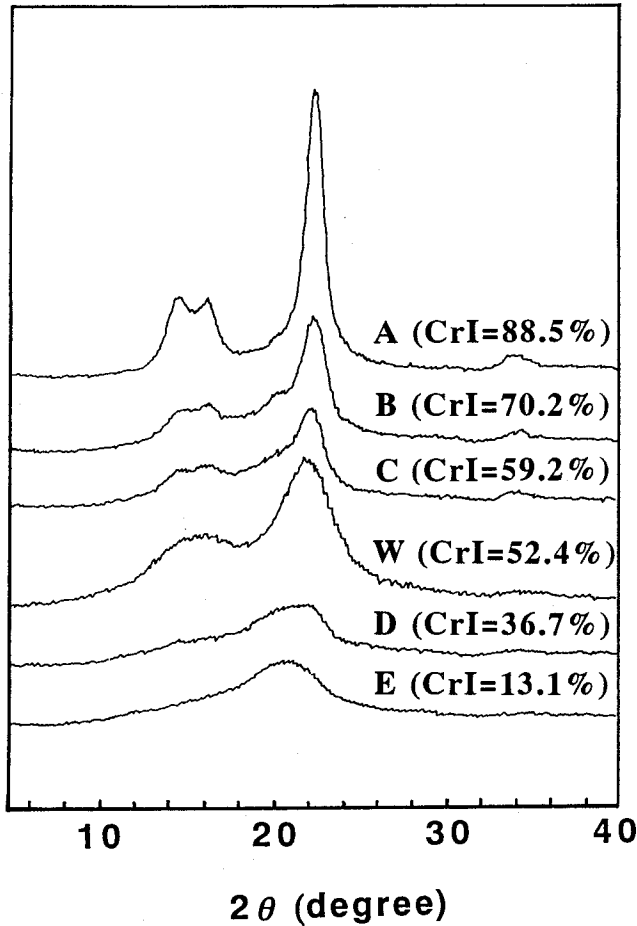
Fig. 7-1. X-ray diffraction diagrams of cellulose substrates. Abbreviations are the same as in Table 7-1.
