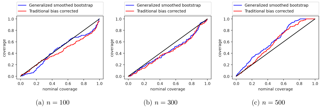
Figure 4: Confidence intervals using bandwidth selected by cross-validation.
