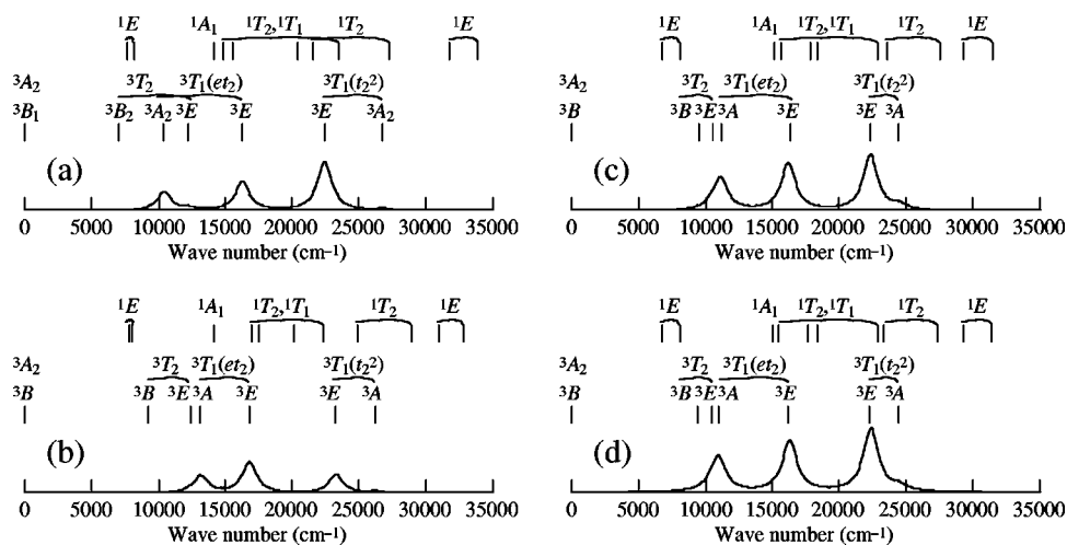
FIG. 5. The calculated multiplet energies and the theoretical absorption spectra obtained from models (a)–(d) by the CDC approach.
