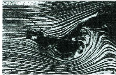
Photo 3 The scene of the wind tunnel experiment recorded on videotape with the high speed camera device
