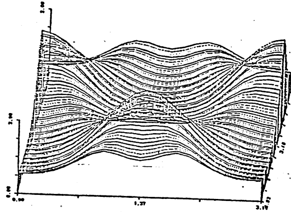
u_2(t, x)
