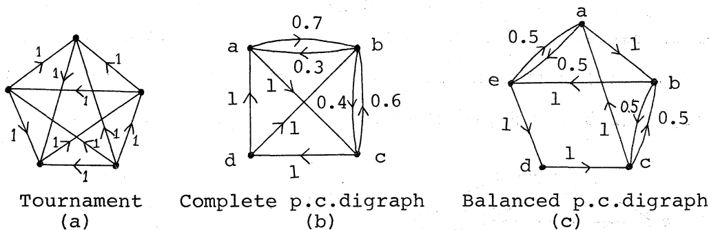
Fig.1 Paired comparison digraphs.
