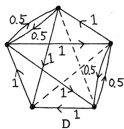
Semi-complete p.c.digraph
