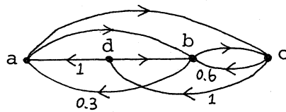
Fig.2 Length of the backward arcs of \alpha .
