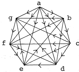
Fig.3 Proper ranks of a complete p.c.digraph.
