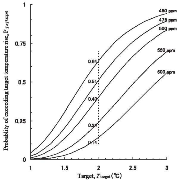
Fig. 2 Probability of exceeding target temperature rise
