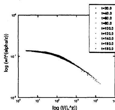
図 2: Results of a data collapse : \alpha = 0.5 , \beta = 0.33 .
