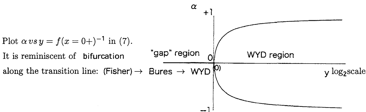
Fig.3 Schematic picture: appearance of the quantum structure of information metrics.
