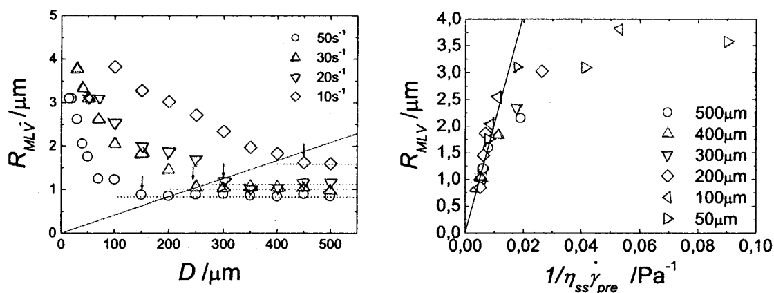
Figure 1: R_{MLV} as a function of gap size, D , (l.h.s.) and R_{MLV} as a function of the inverse of the shear stress, 1/\eta\dot{\gamma} (r.h.s.).
