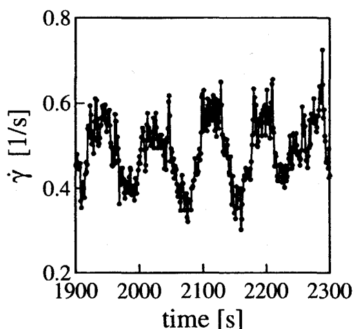
Figure 1: Time evolution of the shear rate for \phi = 35 wt%, T = 339 K and \sigma = 0.2 Pa.
