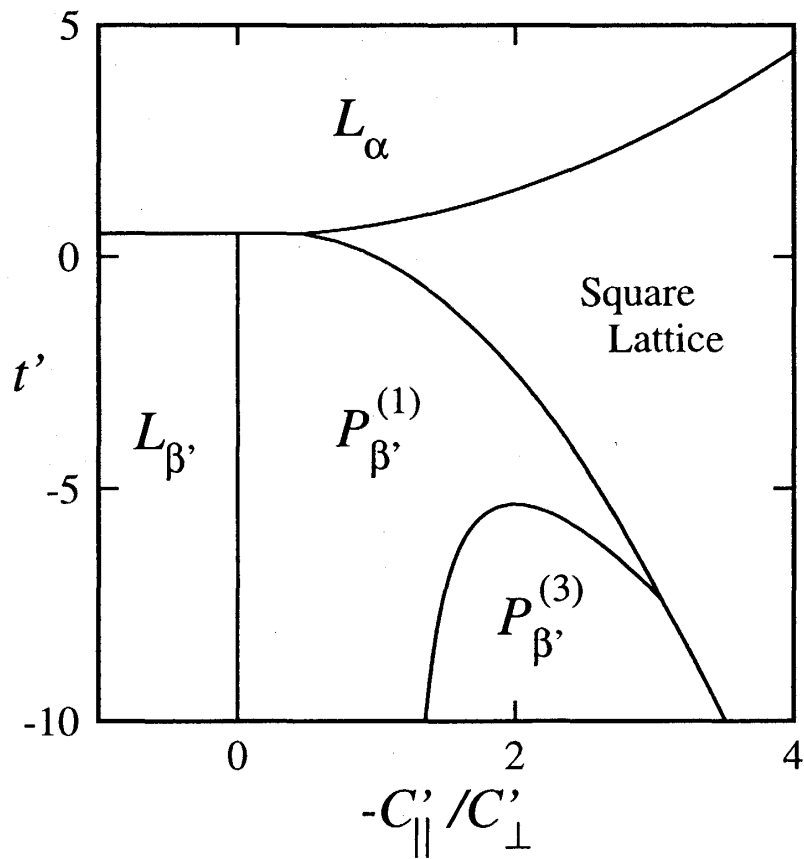
Figure 1: The calculated phase diagram of a single component lipid membrane as a function of the reduced temperature t' and the reduced elastic constant -C'_{\parallel}/C'_{\perp} . L_{\alpha} is the disordered liquid phase, L_{\beta'} is the ordered solid phase, P_{\beta'}^{(1)} and P_{\beta'}^{(3)} are the 1D modulated phases, and the square lattice phase is the 2D modulated phase.
