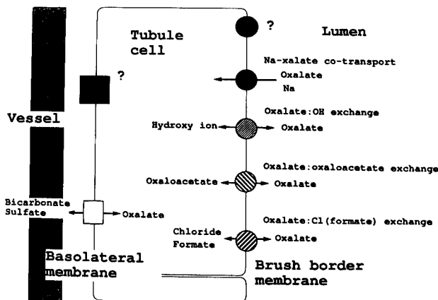
Fig. 2. Oxalate transport systems in the proximal tubule cell.
