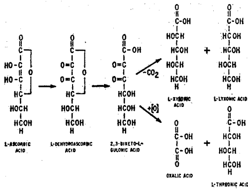
Fig. 8 Pathways of L-ascorbic acid metabolism to form oxalic acid.
