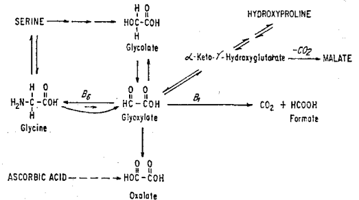
Fig. 7 Major pathways in glyoxylate metabolism and oxalate synthesis in mammalian systems.
