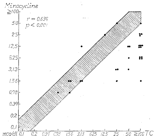
Fig. 7. Cross resistance between minocycline and TC ( E. coli )
