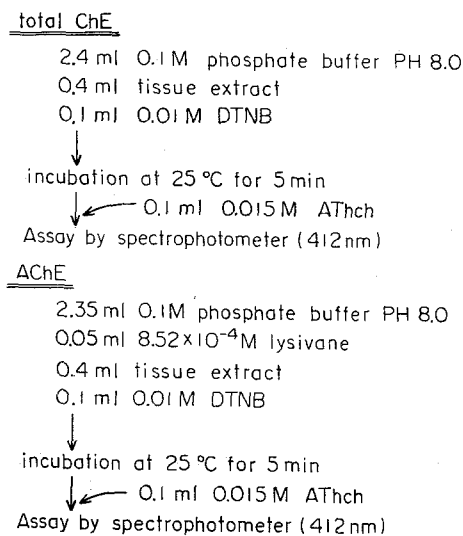
Fig. 2. Assay method
