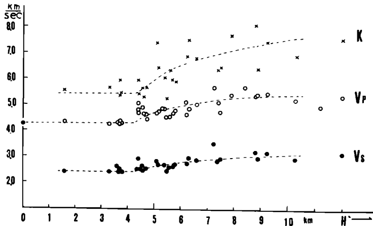
Fig. 3. Wave velocities versus focal depth.
