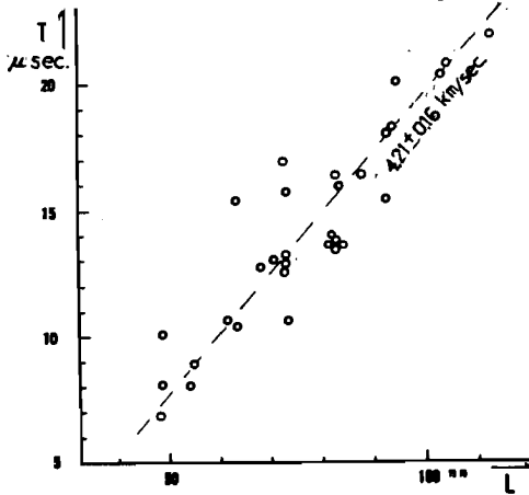
Fig. 4. Transmission times against material's length.
