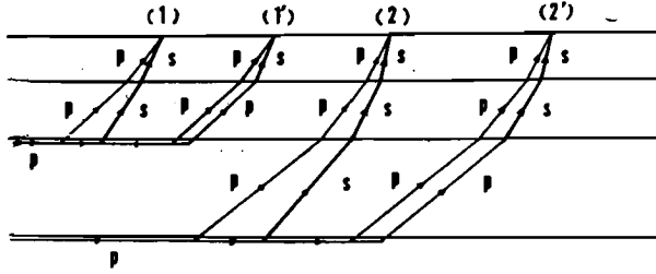
Fig. 9. Schematic representation of wave paths for transformed waves.
